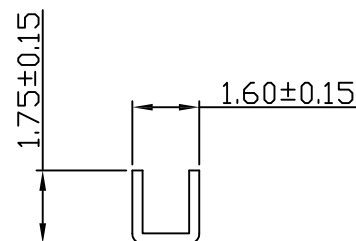
Section: D-D
